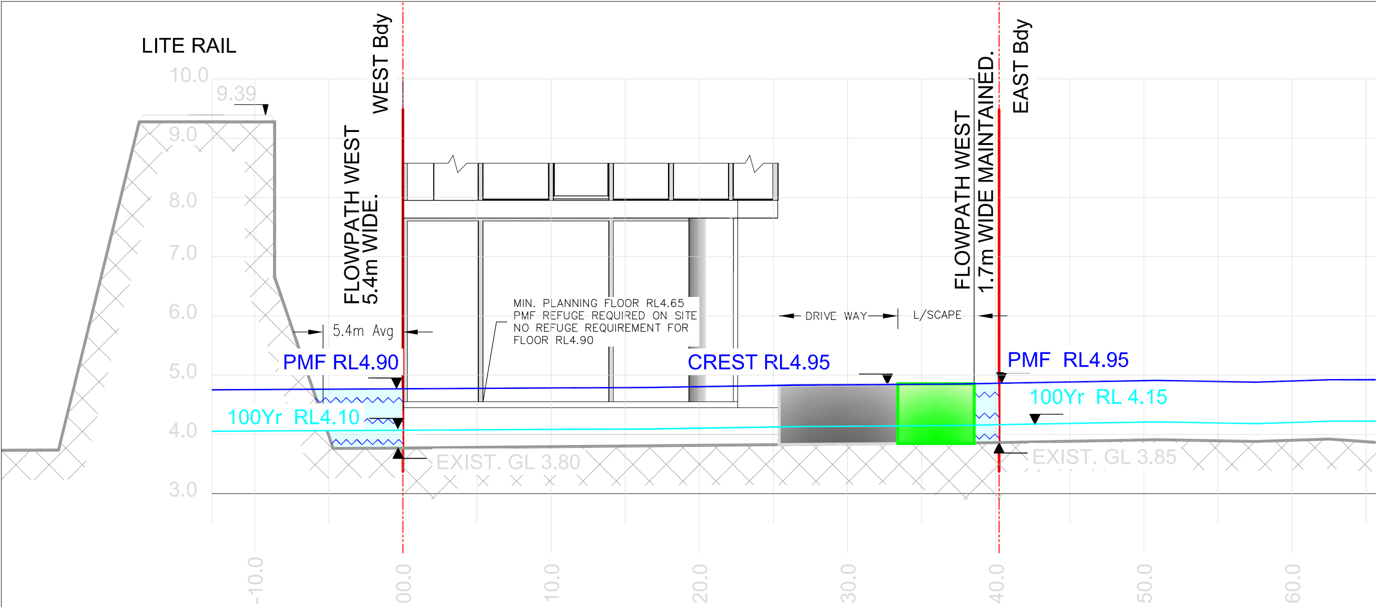
POTENTIAL BUILDING ELEVATION MARION ST. Scale 1:250H, 1: 62.5V
