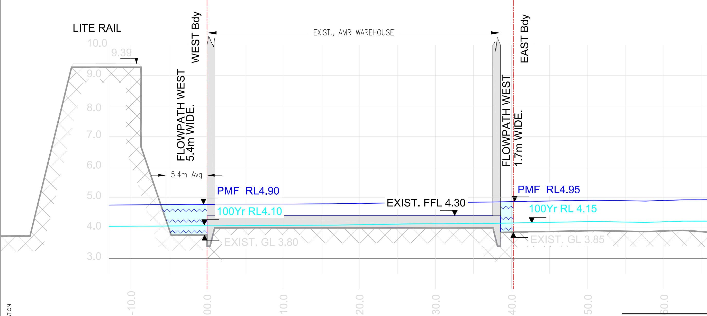
EXISTING ELEVATION MARION ST.
